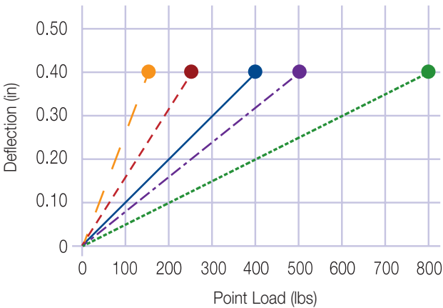
Duo Anti-splay Washer (used for suspending loads from 1/2" slot)
