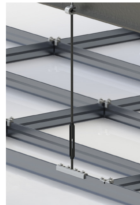
Tate Duo hanging method from steel building
