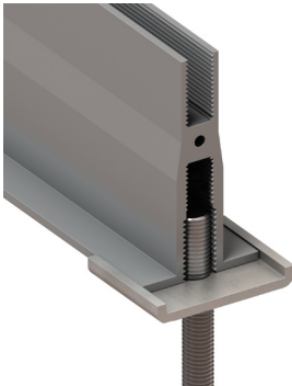
Duo Anti-splay Washer (used for suspending loads from 1/2" slot)
