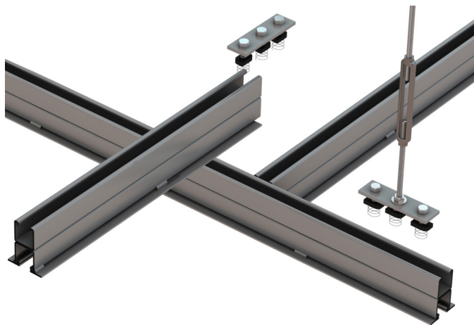
Simple channel nut assemblies are used for strut connections
