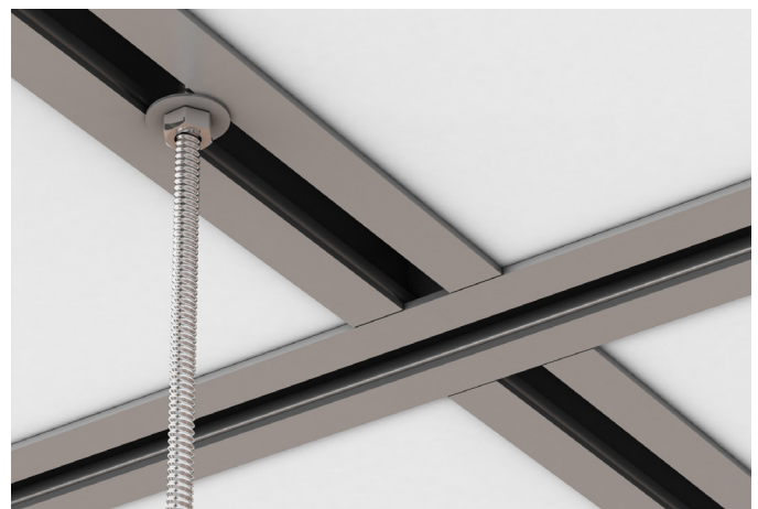
Open slots for connecting cable trays, utilities and other accessories via channel nuts
