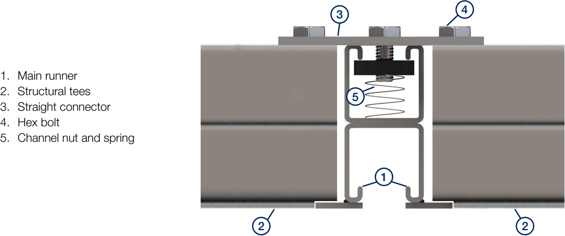
Straight connector joining two structural tees on either side of a main runner. Note all structural tees have factory coped ends
