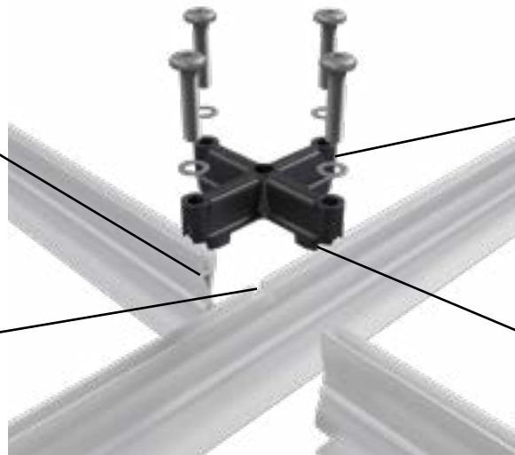
Structural Tee coped for simplified installation and stronger connections
