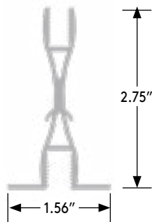
Mains, Tees and Floating Perimeter
