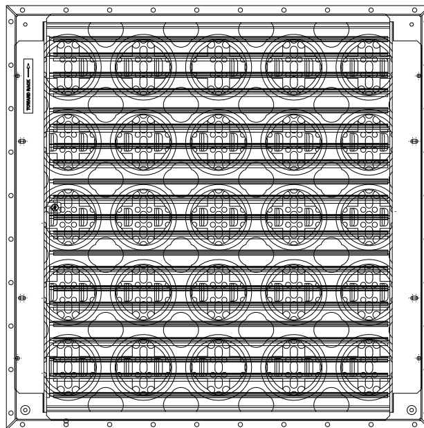
BOTTOM VIEW WITH OPTIONAL OPPOSED BLADE DAMPER
