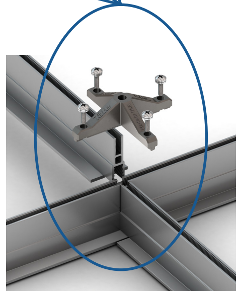
Structural Tee Connections Field Connector (PN39563) 1/4\"-20 Screw with 1/4\" Lock Washer (PN41788)
