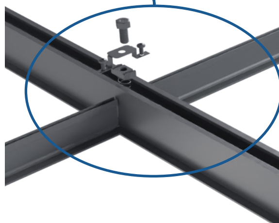
Light Structural to Alustra Connection Light Structural Bridge Connector (PN44246) 1/2" Spring Nut (PN24237) 1/2"-13 x 1" BOLT (PN44324) 1/4" Bolts with 1/4" Washers (PN41788)
