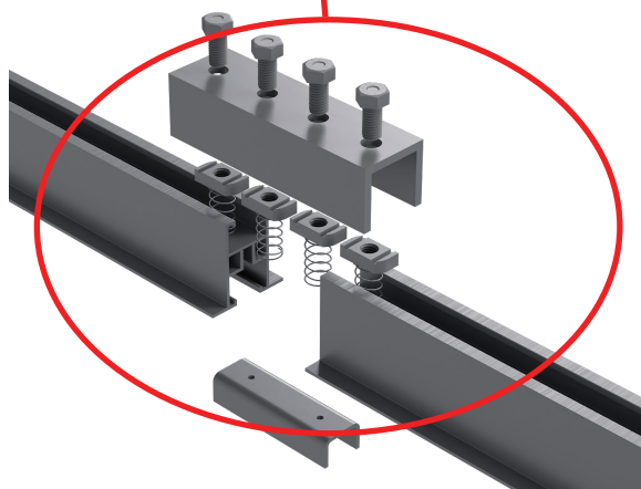
Main Runner Splice Alustra Wrap Around Bracket (PN24244) 1/2" Spring Nut (PN24237) 1/2" -13 x 1" BOLT (PN44324) Splice Bracket (PN44323) 3/8"-16 UNC x 3/4" BHC Screw (PN27099)
