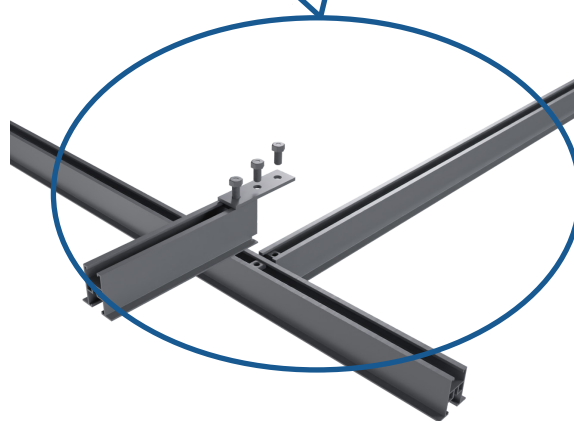
Alustra Cross Tee Connection 3 Hole Straight Bracket (PN24242) 1/2" Spring Nut (PN24237) 1/2" -13 x 1" BOLT (PN44324)
